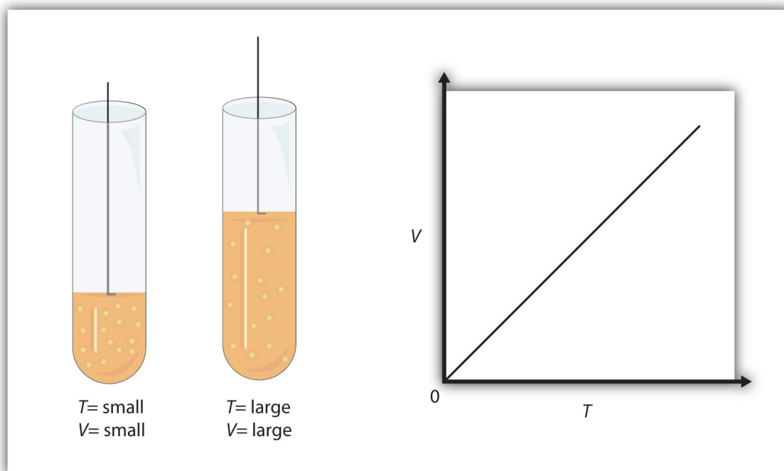
Figure 6.3 Charles's Law
